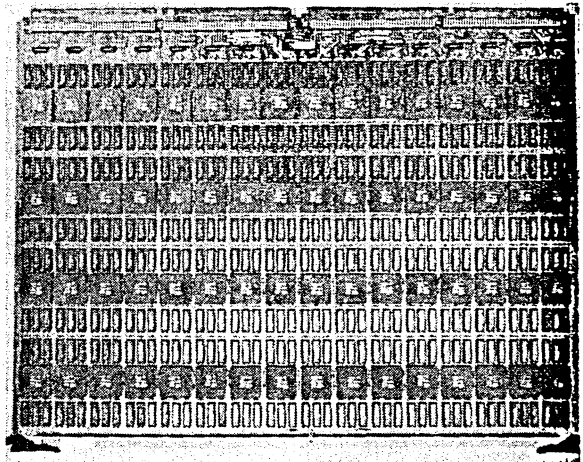
Fig. 3. 64-node NCUBE/ten processor board.
